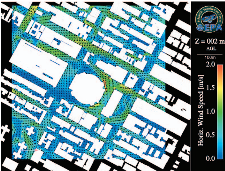
FIG. 8. Simulations of horizontal wind vectors ( \text{m s}^{-1} ) at z = 2 \text{ m} by FLUENT-EPA model for 10 Mar 2005 upstream wind inputs (flow from the northwest).
