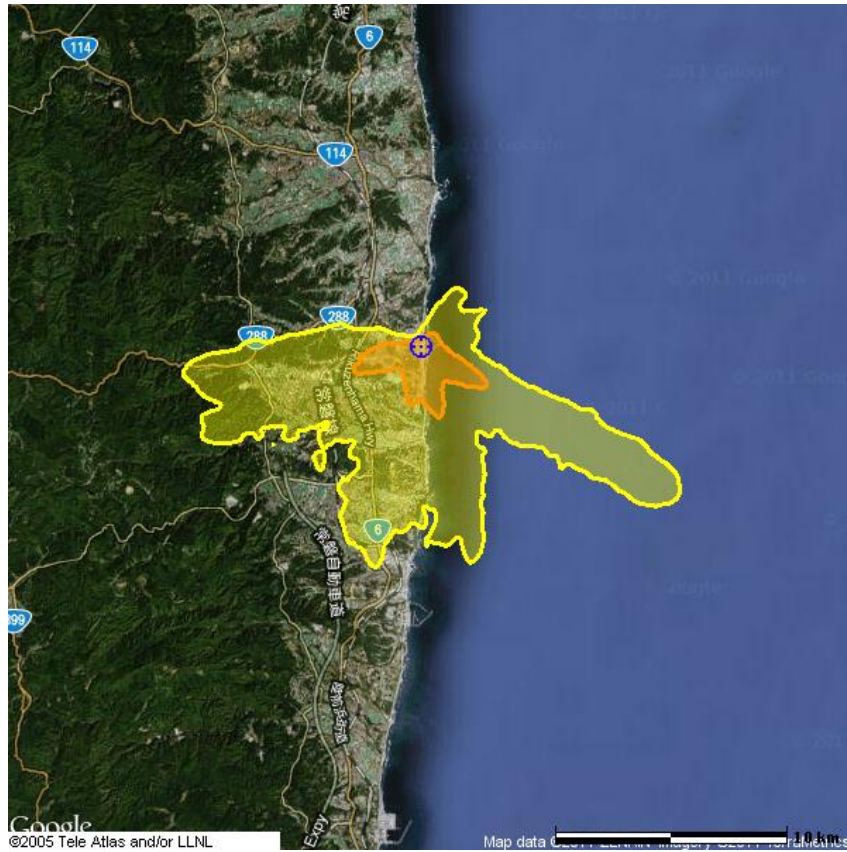
Fig. 1. This figure shows the results of a NARAC ADAPT/LODI simulation of Total Effective Dose (TED) over a 14-day period from 12 March to 26 March 2011 for a hypothetical reactor release scenario provided by the Nuclear Regulatory Commission. The orange and yellow color-filled contours show the areas where the dose is predicted to exceed 0.05 Sv (5 rem) and 0.01 Sv (1 rem), respectively. The top 20 radionuclide contributors to dose and WRF-generated meteorological fields were used in this simulation.
