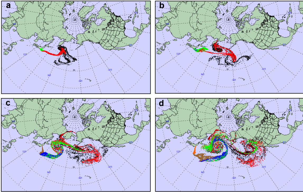
Fig 2. The panels show four frames from an animation of the trans-Pacific transport and dispersion of marker particles from a LODI model simulation of hypothetical releases from the Fukushima Dai-ichi plant. Particle locations are shown for four times: (a) 00:30 UTC 15 March 2011, (b) 00:30 UTC 16 March 2011, (c) 00:30 UTC 17 March 2011 and (d) 00:30 UTC 18 March 2011. Particles of the same color were released during the same 24-hour interval.
