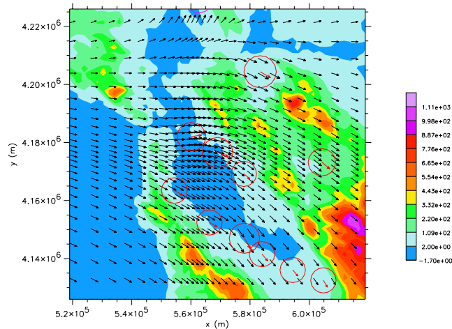
Figure 6: Surface wind field on a graded mesh at 10 m AGL for the same data as in the previous figure. Every third wind vector is plotted.
