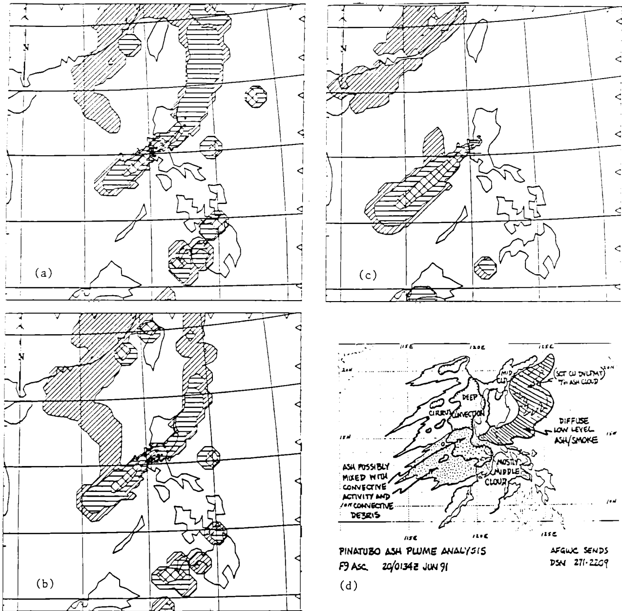
Figure 8 a–d. The relative ash concentration isopleths for three altitude layers a) 5,000–10,000 ft.; b) 10,000–20,000 ft. and c) 20,000–30,000 ft.; d) provides an AFGWC realtime satellite cloud and ash analysis which serves as a verification.
