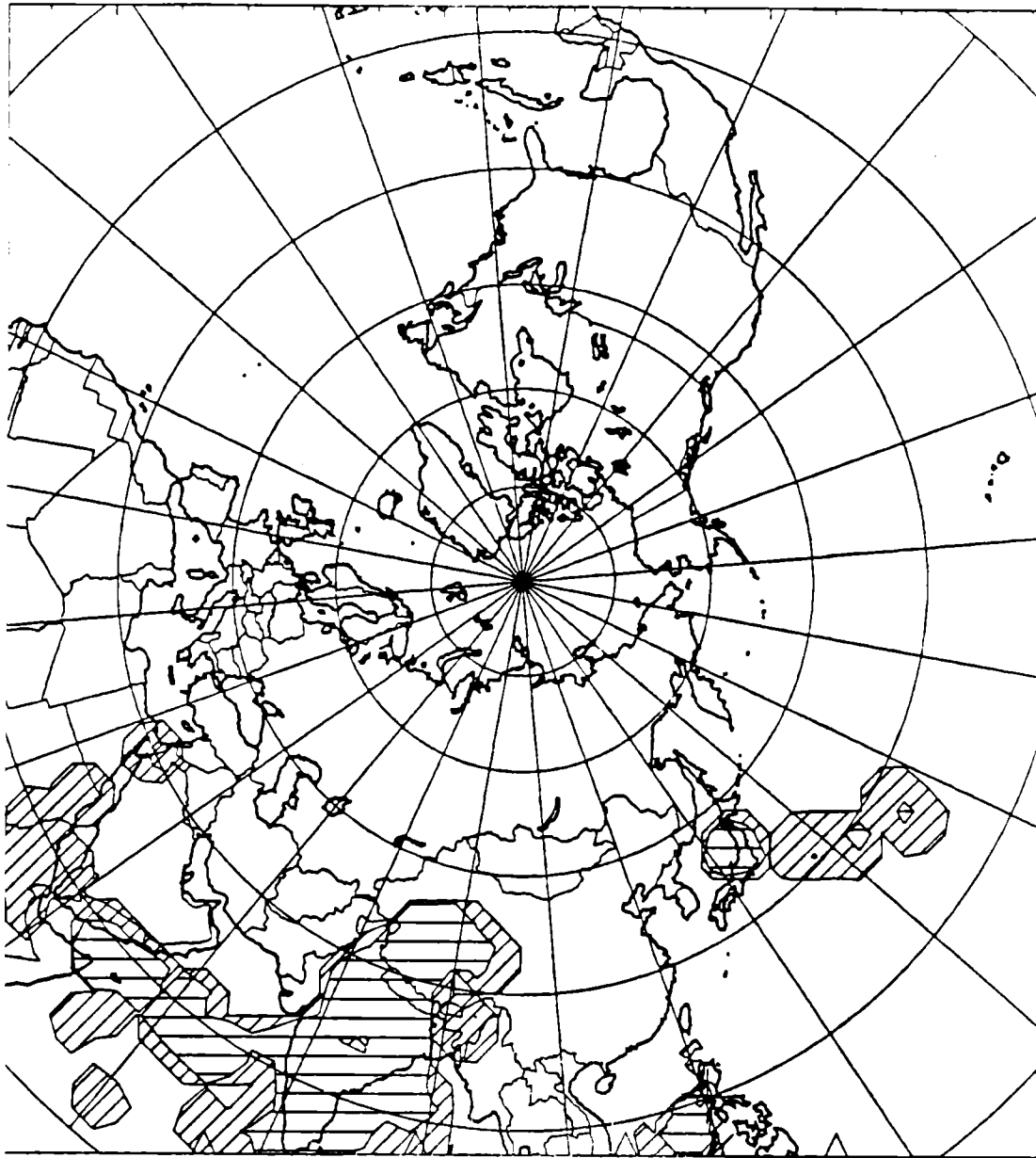
Figure 4. An example of first “ash cloud advisory” map prepared for the USAF on a hemispheric scale. This plot was for the 20–30,000 feet altitude layer valid at 0000 GMT, 20 June 1991. The “ash” levels are relative to the initial release as discussed in the text.
