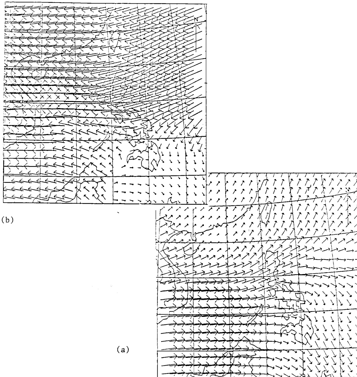
Figure 6a, b. Details of the regional calculations for the 19 June 1991 eruption event (during the U.S. military air evacuations); a) lower atmosphere (2500 m, ~ 7500 ft.) winds; b) upper atmosphere (15,000 m, ~ 50,000 ft) winds.
