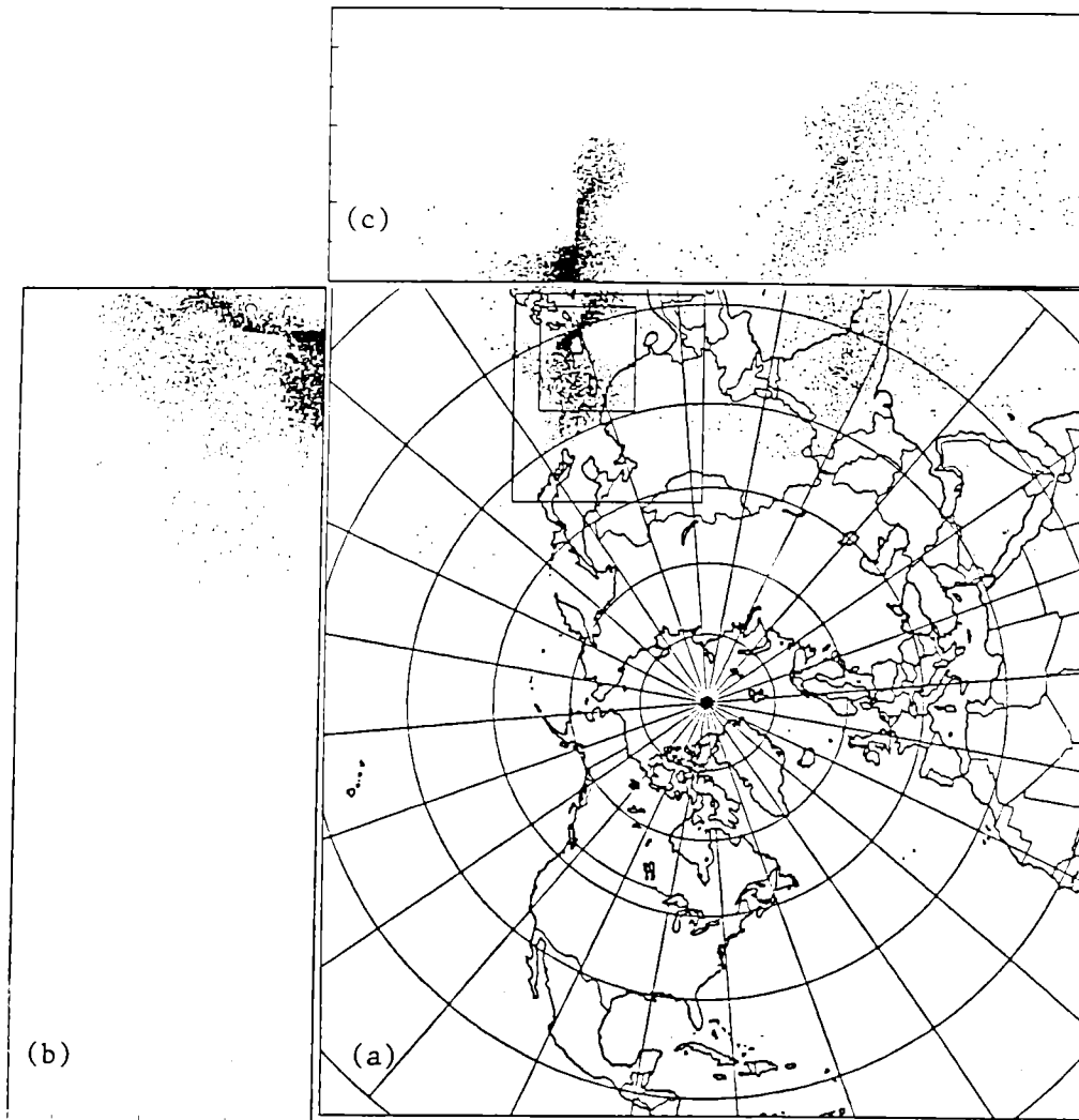
Figures 5a, b, and c. The particle model representation of the dispersing ash clouds for all eruptions from 12–20 June 1991, including the most recent eruption of 1425 GMT on 19 June 1991; a) overhead view; b) side view from right to left of the overhead view, i.e., down the axis of the plume and c) side view from bottom to top (or across the pole) of the overhead revealing the vertical structure of the recent eruption and the more dispersed debris from the cataclysmic eruption (of 15 June 1991) over India (grid top extends to 35,000m).
