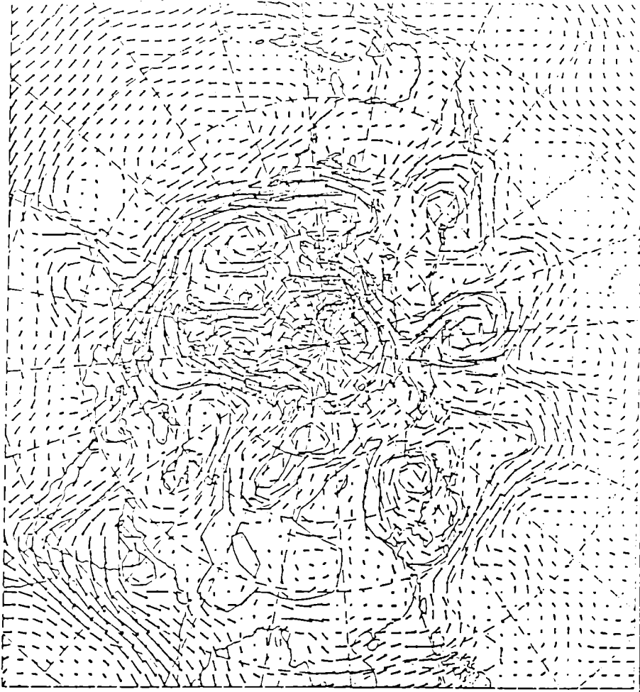
Figure 2. Typical 700 mb (H Pa) level wind field for 20 June 1991 at 0000 GMT.
