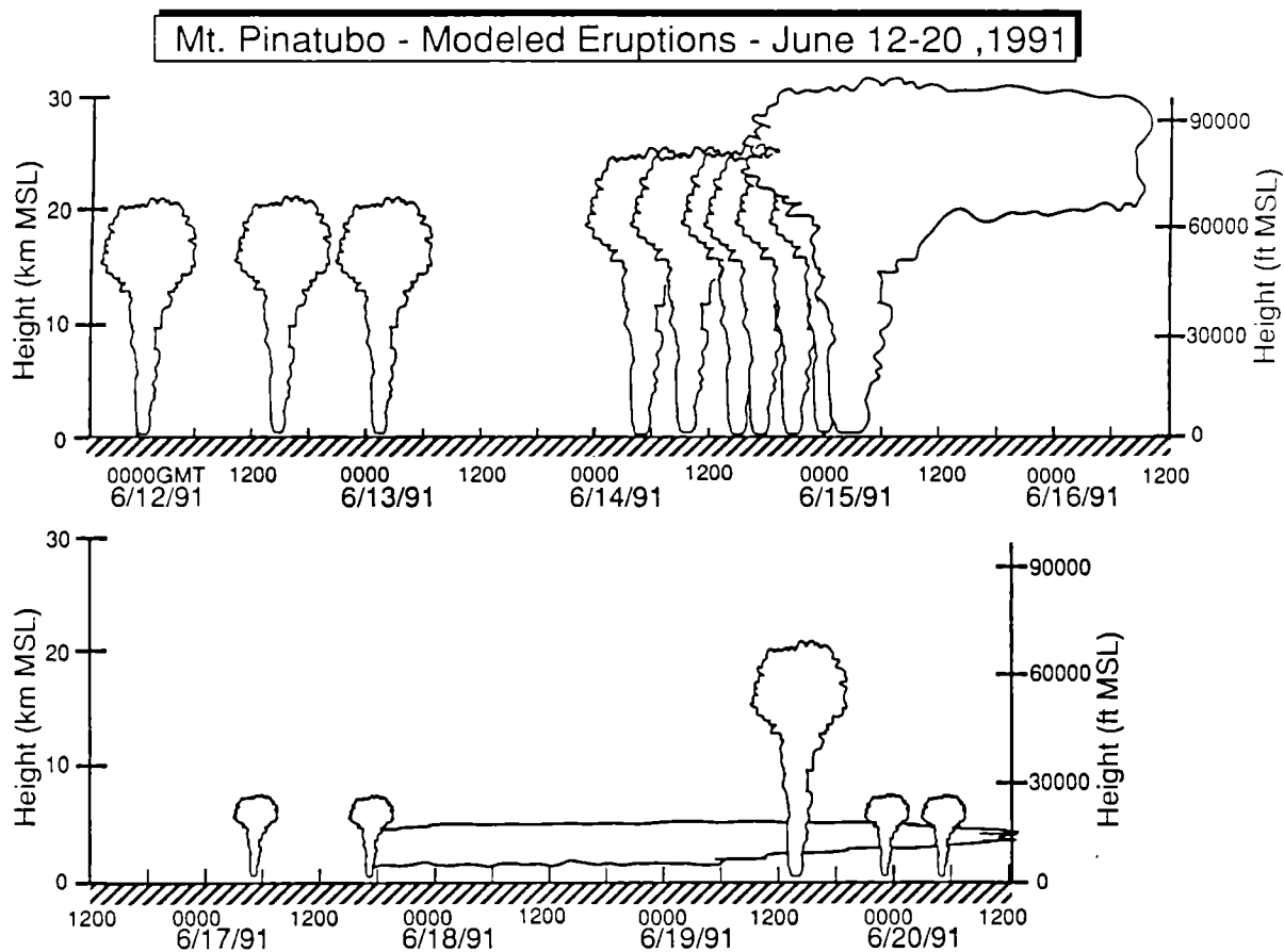
Figure 3. Time sequence and relative eruption heights of events included in the ARAC ash cloud model calculations for the period 12-20 June 1991
