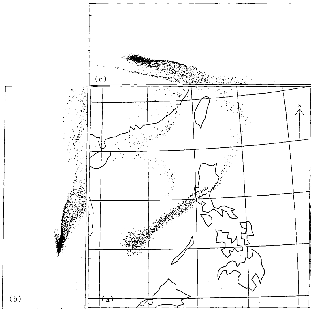
Figure 7. a) Overhead "particle cloud" view for the regional grid calculations of the 19 June 1991 eruption; b) viewed from east to west and c) viewed from south to north.
